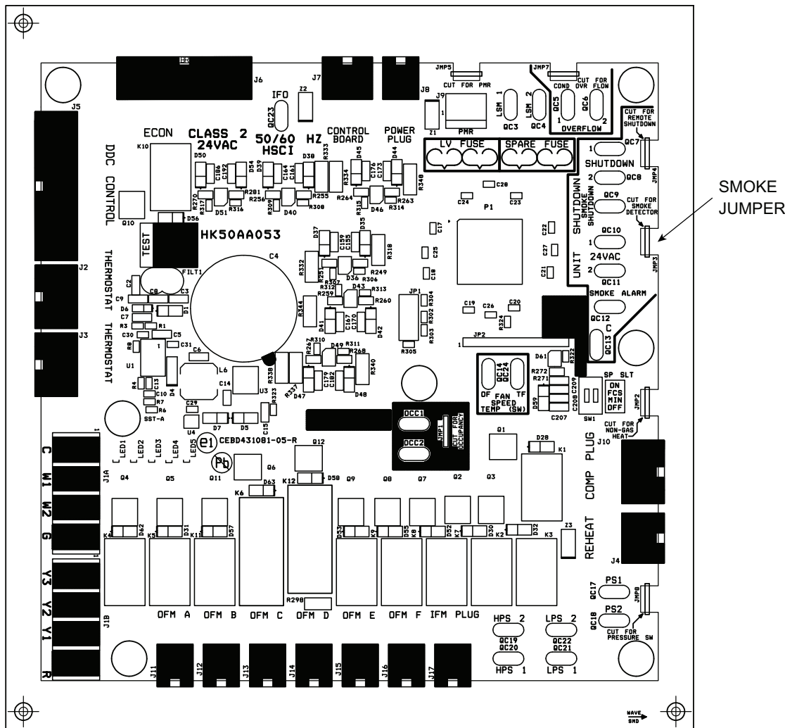
Fig. 11 — 48/50LC Control Board
