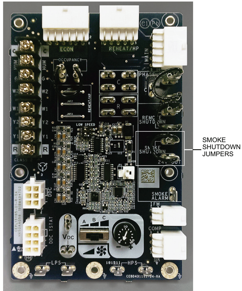
Fig. 10 — Unit Control Board
