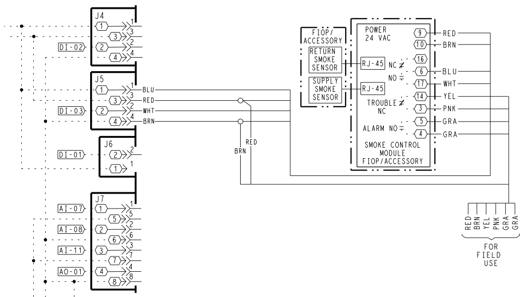
Fig. 5 — SystemVu™ Smoke Detector Wiring
