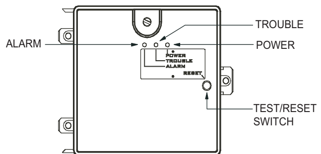
Fig. 3 — Controller Assembly
