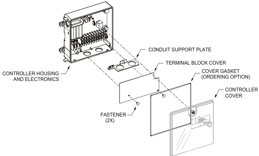
Fig. 1 — Controller Exploded View
