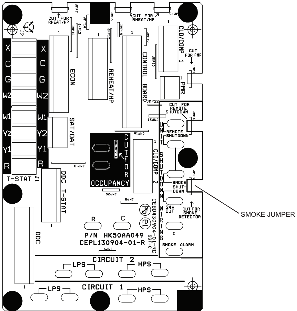
Fig. 9 — Central Terminal Board (Not Used for 48/50LC Models)
