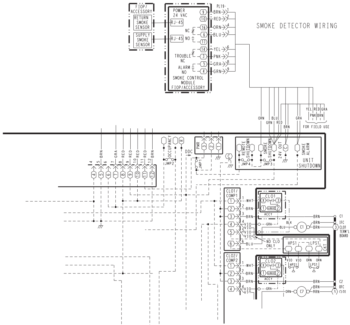
Fig. 4 — Smoke Detector Wiring (Not Used for 48/50LC Models)
